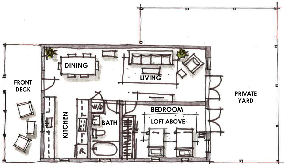
6737 Sueno Road - Sample Floorplan (32' x 22' = 704sf, same plan for all 10 units)
