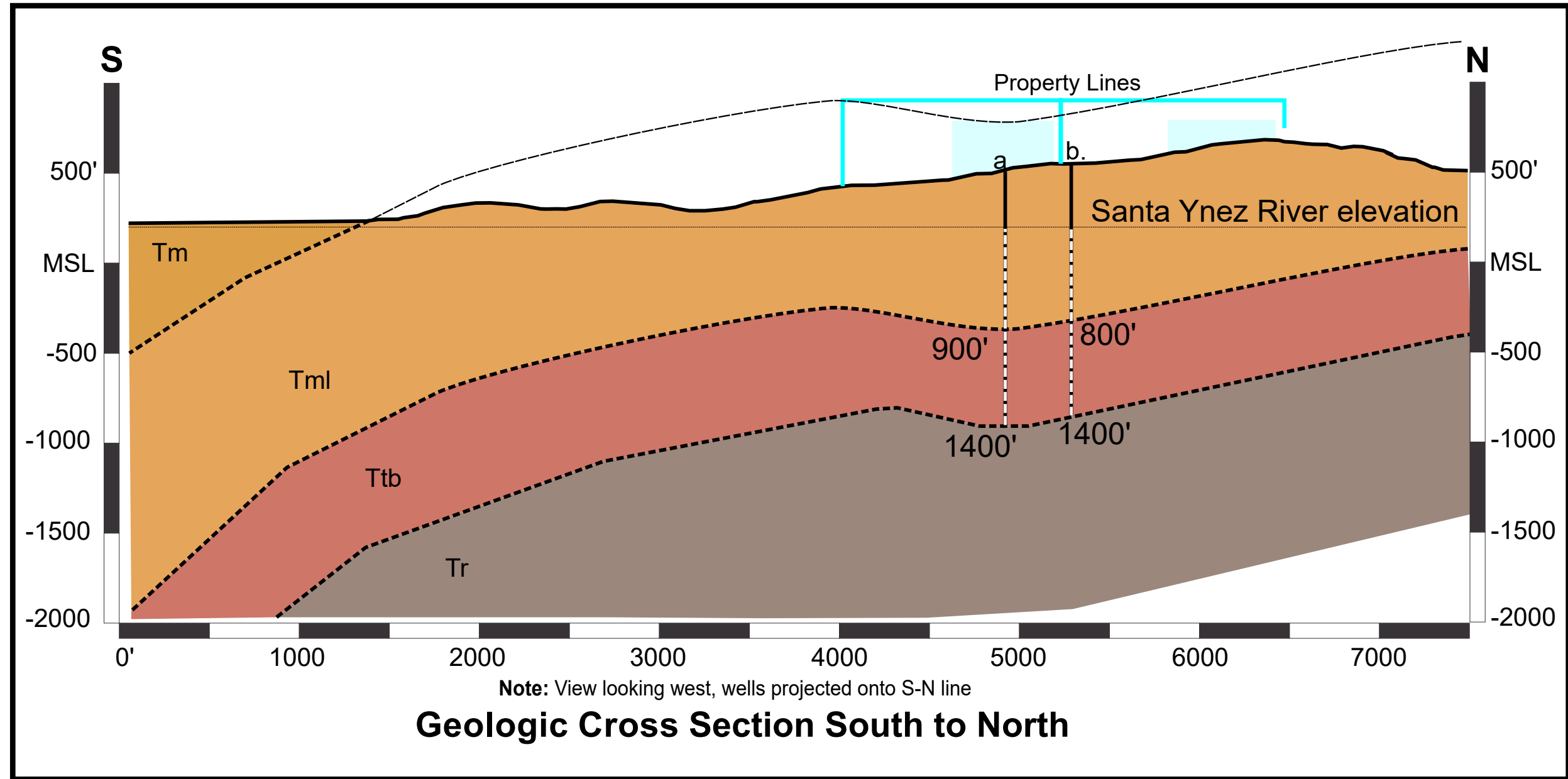
Figure 5 - Geologic cross section underlying Subject Property with recommended well locations. August 2019 KG19-0482
